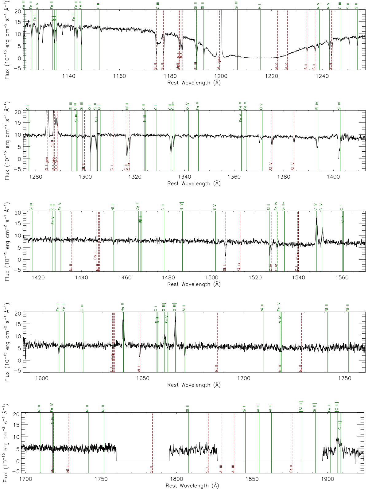
Figure 2. Archival G130M (PI: Aloisi, PID 11579) and new G160M + G185M (PI: Wofford, PID 13788) COS spectroscopy of SBS 0335–052E. From top to bottom we show G130M/seg B, G130M/seg A, G160M/seg B, G160M/seg A, and G185M/seg A+B+C. The spectra are corrected for foreground reddening and redshift, and smoothed to the effective spectral resolution of the G160M data, i.e. 0.51 \text{ \AA} . Intrinsic spectral features are marked with solid-green lines and labelled at the top of each panel. Foreground features are marked with dashed-brown lines and labelled at the bottom of each panel. We use the line list of James et al. (2014) below 1160 \text{ \AA} and that of Leitherer et al. (2011) above 1160 \text{ \AA} . Note the detection of blueshifted \text{O V } \lambda 1371 (plausibly from VMSs), photospheric \text{S V } \lambda 1502 from massive stars, and nebular high-ionization UV emission lines.
