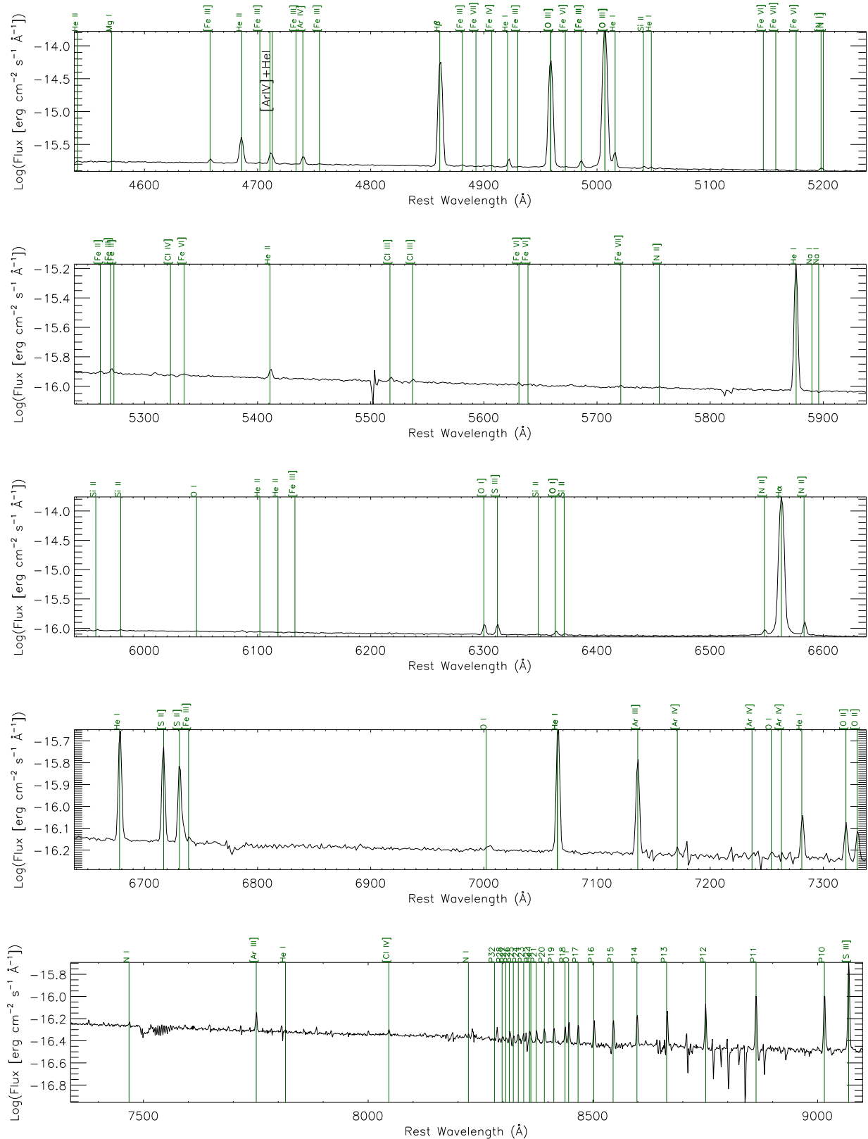
Figure 3. MUSE spectrum of SBS 0335–052E integrated over the COS aperture. The data are plotted with a sampling of 1.23 \text{ \AA} and corrected for foreground reddening and redshift. Intrinsic spectral features are marked with solid-green lines and labelled at the top of each panel. We use the line list of Izotov et al. (2006). Note that some of the absorption, especially in the red part of the spectrum, is caused by residuals of the sky-subtraction procedure from the pipeline. We have, as of yet, made no attempt to correct for this. The same holds for the absorption feature at 7500\text{--}7600 \text{ \AA} , which is a telluric absorption band.
