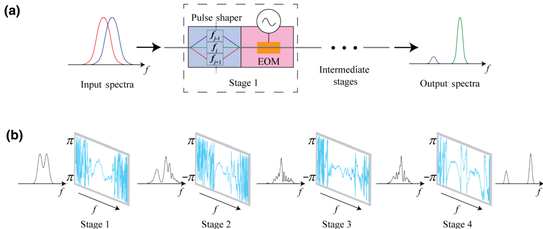
FIG. 2. (a) Schematic of spectrotemporal shaping with optimized spectral phase masks and fixed sinusoidal modulation. The fundamental and orthogonal higher-order HG modes of the input field are transformed into two well-separated Gaussian modes, respectively. (b) Example results for a four-stage spectrotemporal shaping, showing the applied spectral phase masks (blue) and output spectrum distribution (black) at each stage. The modulation depth for all stages is 2.5\pi . The frequency separation between input spectral modes is \delta = \sigma . The fixed temporal modulation at each stage is hidden for convenience.
