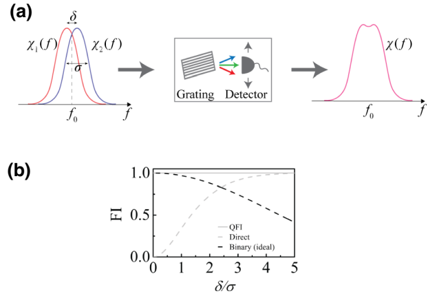
FIG. 1. (a) Schematic of a standard frequency measurement approach: two frequency modes with small separation go through dispersive elements followed by direct detection; (b) Fisher information for different approaches to measure frequency separation. Solid gray, quantum Fisher information; dashed gray, dispersive elements with direct detection; dashed black, binary HG mode detection.
