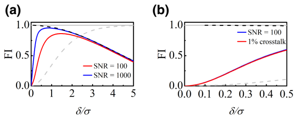
FIG. 7. (a) Fisher information against frequency separation for binary sorting with thermal noise of varied average photon number; (b) comparison between Fisher information versus \delta curves for binary sorting with noise ( \mu = 100 ) and with 1% crosstalk. The QFI, direct detection Fisher information and ideal binary sorting Fisher information curves are replicated from Fig. 1.
