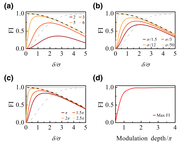
FIG. 3. Fisher information versus frequency separation optimized with (a) different numbers of transformation stages; (b) different frequency resolutions of phase masks; and (c) modulation depths. Quantum Fisher information (solid gray), Fisher information of direct detection (dashed gray), and ideal binary detection (dashed black) are also shown in (a)–(c). (d) Maximum achievable Fisher information with different modulation depths. Except specified, modulation depth is 2.5\pi , frequency resolution for phase masks is infinite, and the number of transformation stages is six.
