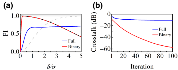
FIG. 6. (a) Fisher information versus frequency separation for full and binary HG mode transformation. Both optimizations are performed with seven stages and modulation depth 2.5\pi . The QFI, direct detection Fisher information and ideal binary sorting Fisher information curves are replicated from Fig. 1; (b) modal crosstalk versus optimization iterations for full and binary transformation schemes.
