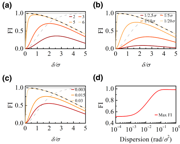
FIG. 5. Fisher information versus frequency separation optimized with (a) different numbers of transformation stages; (b) different temporal resolution of arbitrary wave modulation; and (c) total dispersion. Quantum Fisher information (solid gray), Fisher information of direct detection (dashed gray), and ideal binary transformation (dashed black) are also shown in (a)–(c). (d) Maximum achievable Fisher information with different total dispersion. Except specified, total dispersion is 0.03/\sigma^2 , bandwidth for arbitrary wave modulations is infinite, and the number of transformation stages is six.
