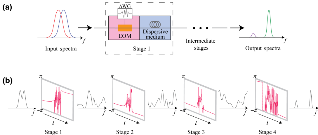
FIG. 4. (a) Schematic of spectrotemporal shaping with optimized temporal modulation and fixed dispersion. The fundamental and orthogonal higher-order HG modes of the input field are transformed into two well-separated Gaussian modes, respectively. (b) Example results for a four-stage spectral-temporal shaping, showing the applied temporal modulation (red) and output spectrum distribution (black) of each stage. Broad spectrum chosen here leads to sharp pulses that require only significant modulation phase change around the center ( t = 0 ) of the time axis. The fixed dispersion for all stages is 0.1/\sigma^2 rad. The frequency separation between input spectral modes is \delta = \sigma . The dispersion phase is hidden for convenience.
