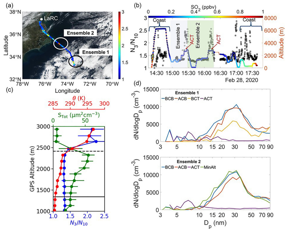
Figure 3. Results from Aerosol Cloud meTeorology Interactions over the western ATLantic Experiment (ACTIVATE) RF10 (February 28, 2020): (a) HU-25 Falcon flight path overlaid on Visible Infrared Imaging Radiometer Suite (VIIRS) imagery (NASA Worldview) with N_3/N_{10} as the color bar. Black and white circles show the approximate location of ensembles 1 and 2, respectively. (b) Time series of N_3/N_{10} (black markers) and aircraft altitude (colored by the MERRA-2 SO_2 ). Shaded regions represent individual cloud ensembles. (c) Vertical profiles of potential temperature, S_{Tot} , and N_3/N_{10} based on data from the descent connecting the above cloud top (ACT) and MinAlt leg during cloud ensemble 1 (15:22:37–15:36:37). Black solid and dashed lines represent cloud base and top heights, respectively. (d) SMPS aerosol number size distributions for different level legs in cloud ensembles 1 and 2.
