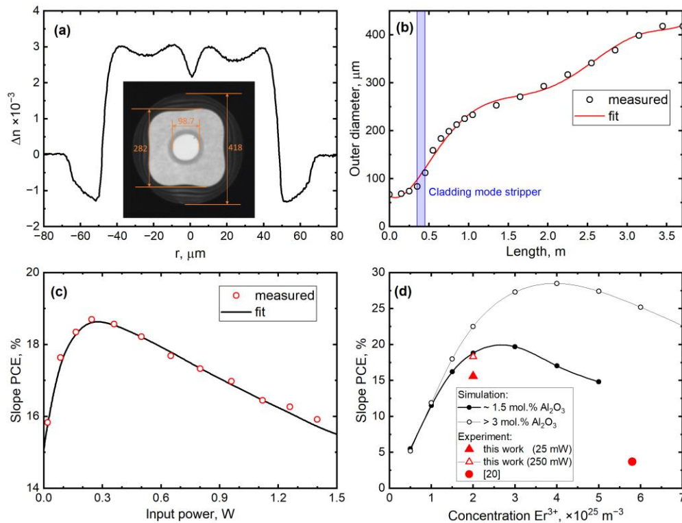
Figure 1. (a) RIP of the T-EDF; inset: photo of the thick end facet; (b) diameter distribution along the T-EDF length (red curve was used in the simulation), the blue bar represents the location of the cladding mode stripper produces on the T-EDF; (c) signal saturation curve of the T-EDF (the circles correspond to measured values and the black curve is an approximation); (d) calculated slope PCE of the T-EDF with clustering curves for different alumina concentrations and experimental data. In (c,d) the signal wavelength was 1555 nm and the pump wavelength was 976 nm.
