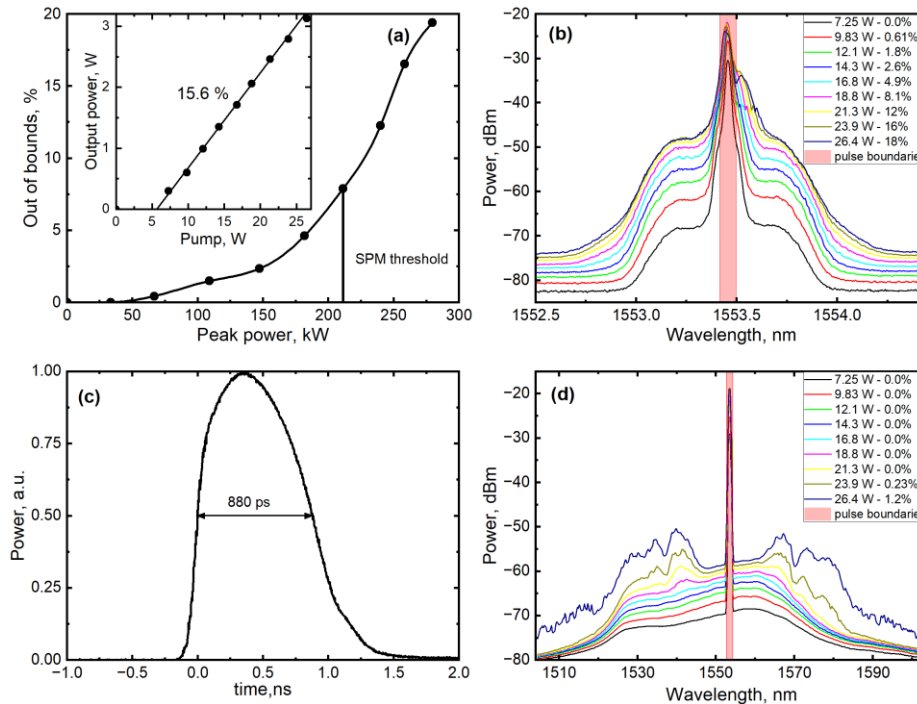
Figure 3. Results of ns pulses amplification in the T-EDF. (a) The out of bounds part of the output power as shown in (b) and (d) vs. peak power; inset: output power vs. pump power; (c) the waveform of the output pulse measured with 50 GHz stroboscopic oscilloscope; (b,d) output spectrum at a resolution of 0.02 nm (b) and 1 nm (d). The red rectangle indicates the part of the spectrum which is considered “in-pulse.” Anything outside the red rectangle is considered to be outside of pulse boundaries for energy and peak power calculations. Pulse boundaries widths are 0.04 nm (b) and 2 nm (d).
