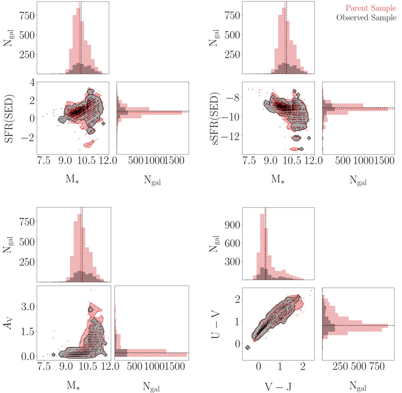
Figure 9. Corner plots for SFR(SED). M_* (upper left), sSFR(SED) versus M_* (upper right), A_V versus M_* (bottom left), and U-V versus V-J (bottom right). Shown on these diagrams are the z \sim 2 parent sample (red) and z \sim 2 observed sample (black). The galaxy properties shown here are estimated using emission-line uncorrected photometry for all galaxies in the figure. The parameter distributions and sample medians are shown in the 1D histogram panels, while the individual data points and 3\sigma shaded contours for each sample are shown in 2D space.
