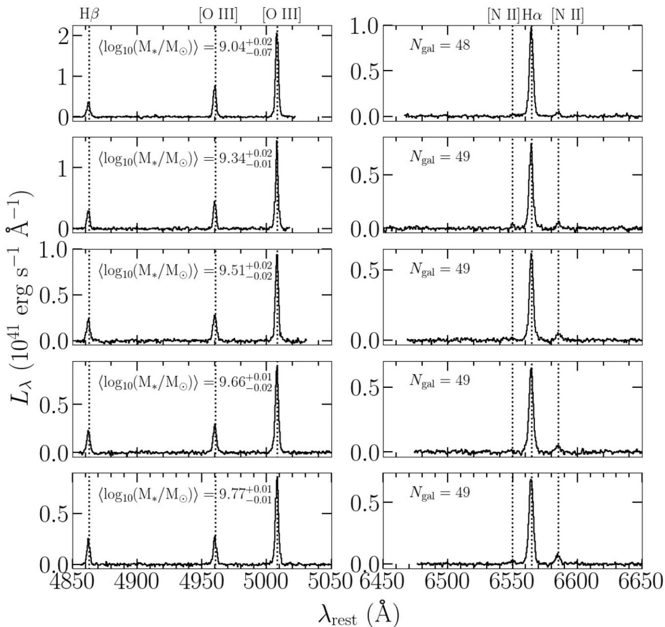
Figure 2. Composite spectra for the five lower- M_* bins in the z \sim 2 N2 stacked sample. The dotted vertical lines identify the rest-optical emission-lines in the stacks. The left-hand panel shows H \beta and [O III] \lambda\lambda 4960, 5008 while the right-hand panel shows H \alpha and [N II] \lambda\lambda 6550, 6585 . The emission lines are labelled in the top panels. The average M_* for each bin is given in the left-hand panels while the number of galaxies in each bin ( N_{\text{gal}} ) is given in the right-hand panels. Note that the limits of the y-axis are adjusted in each panel to best show the emission lines. Also note that the emission lines show a general decrease in flux as the bins increase in M_* , most pronounced for H \beta and [O III] \lambda\lambda 4960, 5008 .
