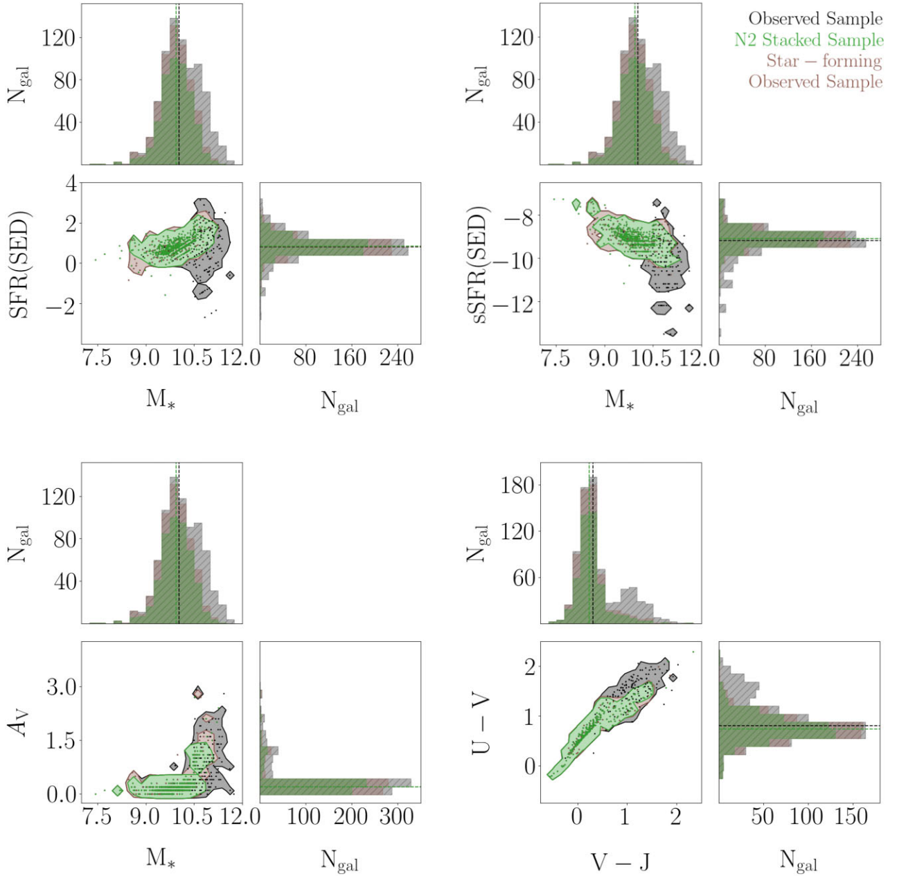
Figure 10. Corner plots for SFR(SED) versus M_* (upper left), sSFR(SED) versus M_* (upper right), A_V versus M_* (bottom left), and U-V versus V-J (bottom right). Shown on these diagrams are the z \sim 2 observed sample (black), z \sim 2 star-forming observed sample (brown), and the z \sim 2 N2 stacked sample (green). The galaxy properties shown here are estimated using emission-line corrected photometry for the majority of the galaxies with a MOSFIRE redshift. Otherwise, emission-line uncorrected photometry is used for the minority of galaxies without the z_{\text{MOSFIRE}} . The parameter distributions and sample medians are shown in the 1D histogram panels, while the individual data points and 3\sigma shaded contours for each sample are shown in 2D space.
