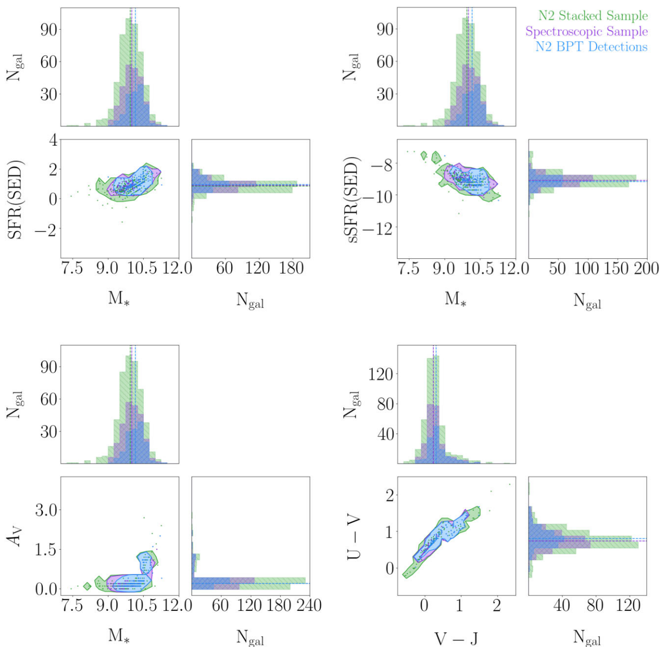
Figure 6. Corner plots for SFR(SED) versus M_* (upper left), sSFR(SED) versus M_* (upper right), A_V versus M_* (bottom left), and U-V versus V-J (bottom right). Shown on these diagrams are the z \sim 2 stacked sample (green), z \sim 2 spectroscopic sample (purple), and z \sim 2 N2 BPT detections (blue). The galaxy properties shown here are estimated using emission-line corrected photometry for all galaxies in the figure. The parameter distributions and sample medians are shown in the 1D histogram panels, while the individual data points and 3\sigma shaded contours for each sample are shown in 2D space.
