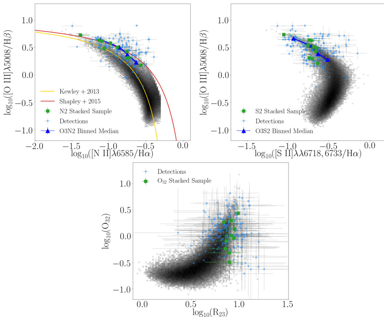
Figure 4. The [N II] BPT (top left), [S II] BPT (top right), and O_{32} versus R_{23} (bottom) diagrams. The N2 and S2 z \sim 2 stacked samples are shown with green squares. The grey 2D histograms show the local SDSS z \sim 0 star-forming galaxies. The blue points identify the 143, 156, and 181 galaxies with 3\sigma S/N for all relevant lines on the [N II] BPT, [S II] BPT, and O_{32} versus R_{23} diagrams, respectively. An additional requirement for a robust H\alpha detection is needed for dust corrections on the O_{32} versus R_{23} diagram. The blue triangles are the binned medians from Runco et al. (2022), binned in O3N2 (O3S2) on the [N II] ([S II]) BPT diagram. The red curve on the [N II] BPT diagram is a fit to early MOSDEF data from Shapley et al. (2015), while the yellow curve is a fit to the SDSS z \sim 0 star-forming locus (Kewley et al. 2013).
