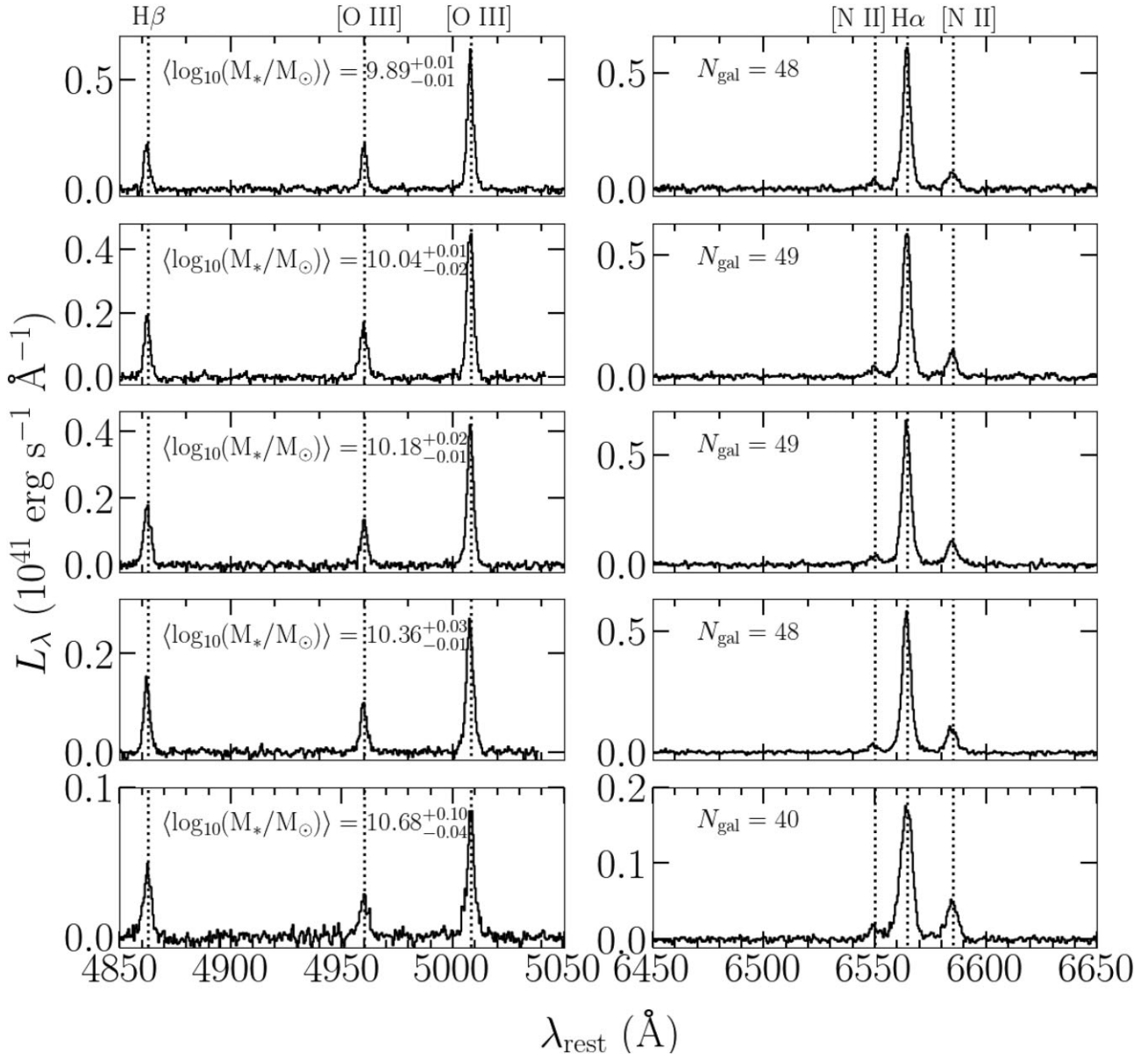
Figure 3. Same as Fig. 2 but displaying the composite spectra for the five higher- M_* bins in the z \sim 2 N2 stacked sample.
