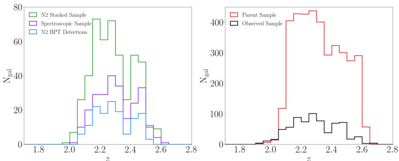
Figure 1. Redshift distributions for the different MOSDEF samples analysed in this study. The left-hand panel shows the MOSDEF z \sim 2 N2 stacked sample (green; z_{\text{med}} = 2.28 ), z \sim 2 spectroscopic sample (purple; z_{\text{med}} = 2.29 ), and z \sim 2 N2 BPT detection sample (blue; z_{\text{med}} = 2.29 ). The right-hand panel shows the MOSDEF z \sim 2 observed sample (black; z_{\text{med}} = 2.29 ) and z \sim 2 parent sample (red; z_{\text{med}} = 2.31 ).
