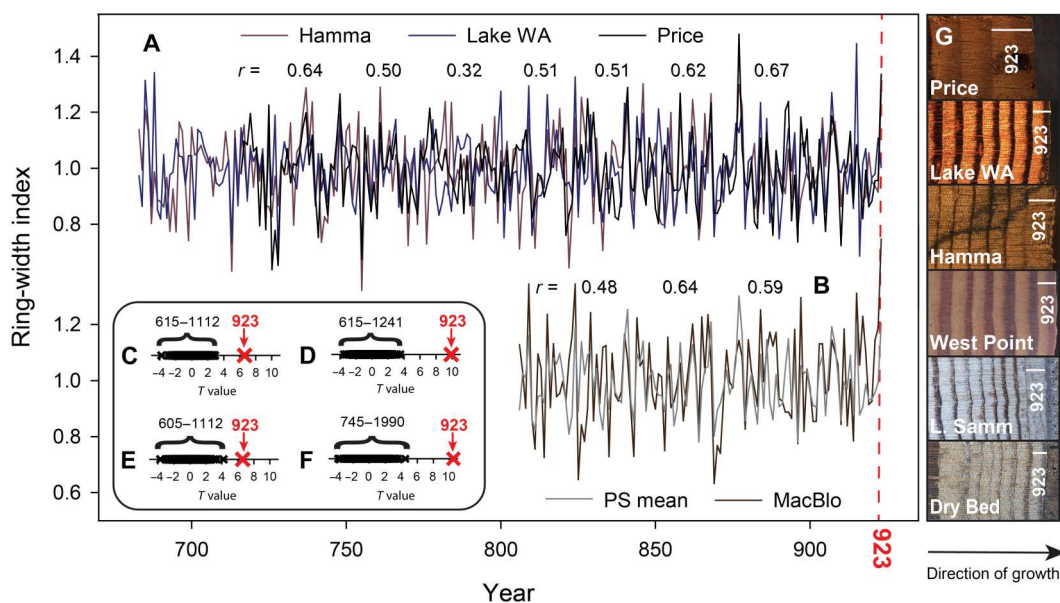
Fig. 2. Tree-ring dating of Puget Sound sites. (A) Site-level tree-ring width chronologies from Hamma Hamma, Lake Washington, and Price Lake. Numbers are running correlation coefficients ( r ) between each chronology and the mean of the other two, as calculated in 50-year windows overlapping by 25 years. (B) Mean of the three Puget Sound chronologies (PS mean) and the MacBlo chronology. Numbers are correlation running coefficients ( r ) between the plotted chronologies calculated in 50-year windows overlapping by 25 years. Inset: Heavy black horizontal bars represent the distribution of T values, a measure of correlation, when sliding each pair of chronologies back and forth through time relative to one another for (C) Hamma Hamma and Price Lake, (D) Hamma Hamma and Lake Washington, and (E) Lake Washington and Price Lake and (F) MacBlo and PS mean. T value when ends of chronologies are aligned to 923 is shown as a red "X." Values in brackets are the range of dates (CE) across, which chronologies are compared. (G) Images of the final tree rings from representative samples at all six sites. The final ring corresponds to 923 CE, the width of which is shown by a white line; bark is still attached to the bottom two samples.
