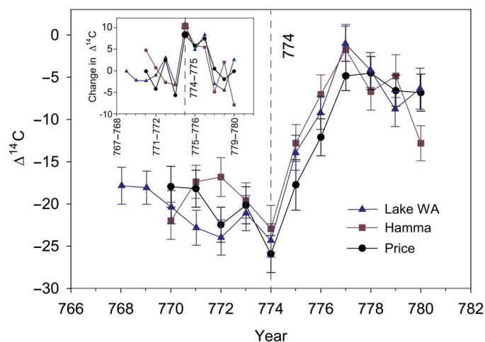
Fig. 3. The 774–775 radiocarbon pulse in Puget Sound tree-ring data. Annual \Delta^{14}\text{C} from tree samples of Hamma Hamma, Lake Washington, and Price Lake. Inset: Difference in \Delta^{14}\text{C} from 1 year to the next to illustrate the magnitude of the jump from 774 to 775 CE (dashed vertical line). An enlarged symbol denotes the year of the largest radiocarbon jump in each time series, which at all three sites occurs from 774 to 775 CE.
