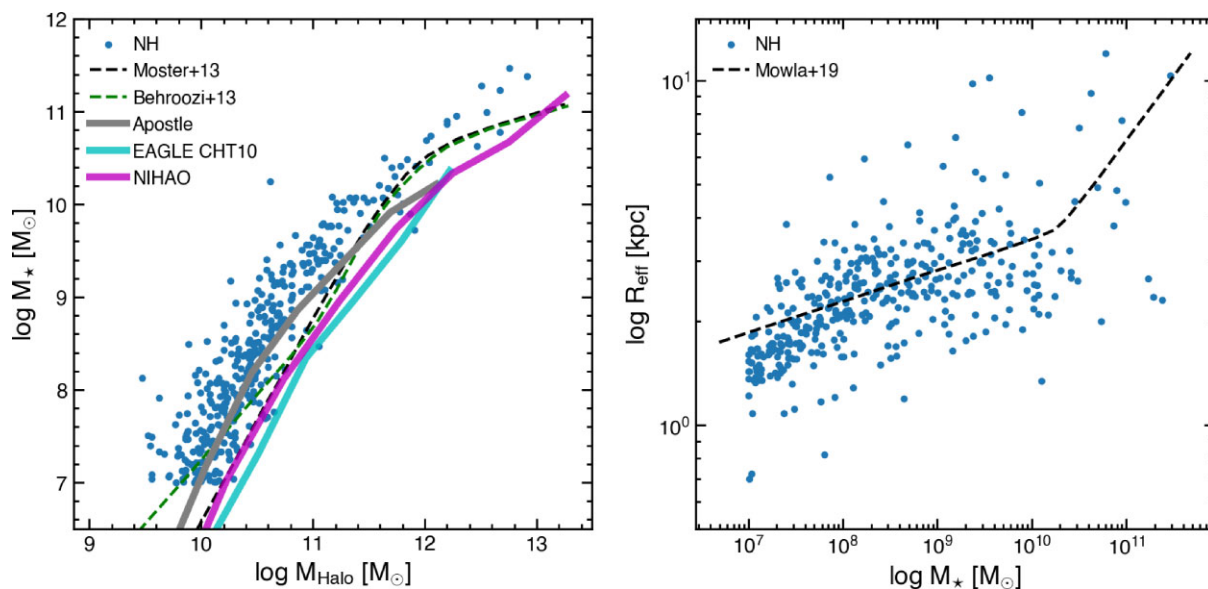
Figure 1. Left: M_{\text{Halo}} versus M_* for the NH galaxy sample used in this study (blue circles). We compare to the abundance matching studies from Behroozi et al. (2013) and Moster et al. (2013) and other simulations: APOSTLE (Sawala et al. 2016), EAGLE CHT10 (Benítez-Llambay et al. 2019), and NIHAO (Wang et al. 2015). On average, NH Haloes contain more stellar mass than other simulations, with the observational data lying between NH and the other simulations. Right: M_* versus R_{\text{eff}} for the NH galaxy sample (blue circles). We also show the best fit observational results from Mowla et al. (2019) ( z = 0.37 ). The sizes of NH galaxies are well-matched to the observations, particularly in the stellar mass range of interest in this study. For more details of how NH matches to observational results, see Dubois et al. (2021).
