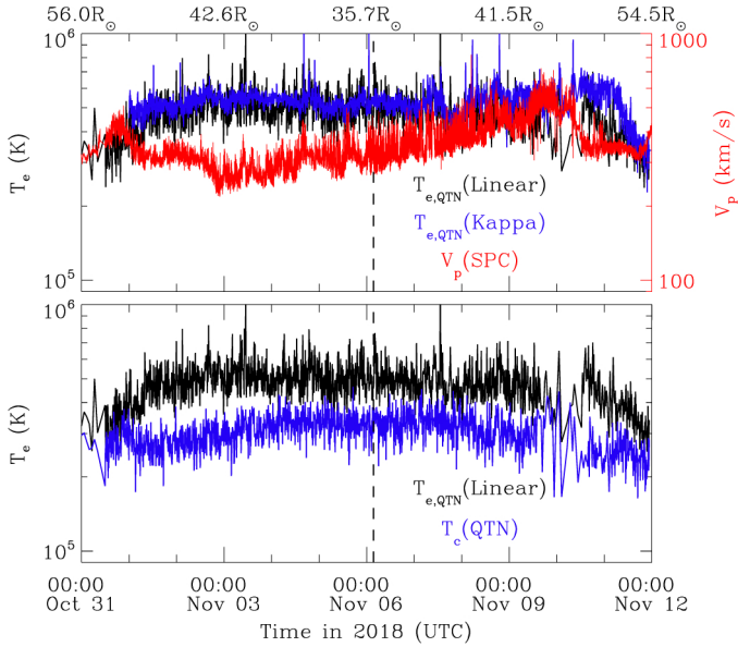
Fig. 2. Comparison of observations of solar wind electron temperatures derived from different methods from PSP. An example of 12-day period of measurements from PSP during encounter one (from October 31, 2018 00:00:00 to November 12, 2018 00:00:00 UTC) is shown for reference. The heliocentric distance (in units of the solar radius R_{\odot} ) is indicated at the top of the top panel and the black vertical line denotes the first perihelion of the PSP orbit. From the top to bottom panels, the total electron temperature derived from the linear fit QTN technique is displayed in black. In the top panel, the total electron temperature obtained by fitting the high-frequency part of the spectrum with the generalized Lorentzian QTN model (Maksimovic et al. 2020) is shown in blue for comparison. The bottom panel follows the same format as the first panel but for the core electron temperature derived from the simplified QTN technique (Moncuquet et al. 2020). The proton bulk speed from SPC/SWEAP is presented in the top panel for reference. An anticorrelation between V_p and T_e , which was also previously reported in Maksimovic et al. (2020), is visible during the time interval considered. We note that we have already smoothed T_{e,QTN}(\text{linear}) , T_{c,QTN} , and T_{e,QTN}(\text{kappa}) , so that the comparison between them is clear.
