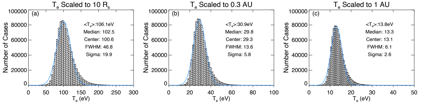
Fig. 4. (a–c): Histograms of the total electron temperature ( T_e ) scaled to 10 solar radii, 0.3 AU and 1 AU, based on observations displayed in Fig. 3 and their corresponding power law modelling fit results. Gaussian fit is superimposed in blue on each histogram. The corresponding average and median values are also indicated together with the center value and 1- \sigma standard deviation of the Gaussian fit.
