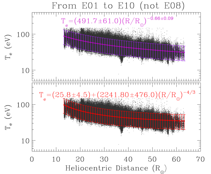
Fig. 3. Radial variation of the total electron temperature ( T_e ) combining observations from encounters one (E01) to ten (E10), with E08 excluded. From top to bottom, T_e is fitted with the power law expression T_e = T_0 \times (R/R_{\odot})^{\beta} (purple) and the expression given by the large distance exospheric solar wind model T_e = T_0 + T_1 \times (R/R_{\odot})^{-4/3} (red), respectively. The fitted profile and expression with corresponding color are superimposed for comparison. The variations of the free parameters in the fitted expressions are the corresponding 1-sigma ( 1-\sigma ) fit uncertainties. The vertical error bars indicate the 2- \sigma fit uncertainties, which covers about 95% data points in total.
