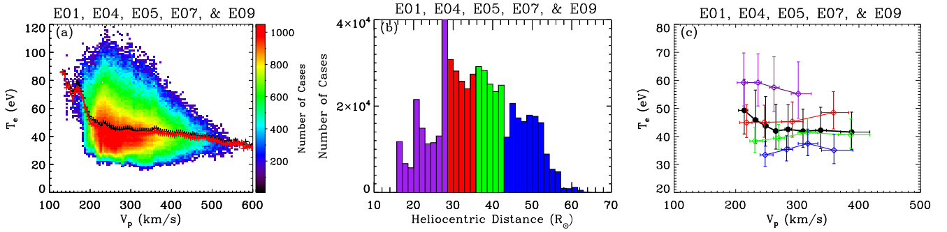
Fig. 7. Illustration of T_e against V_p combining observations from E01, E04, E05, E07, and E09. (a) 2D histogram distribution of T_e versus V_p with the color bar on the right side indicating the number of data points. Both the mean (red curve) and median values (black curve) are superimposed for reference. A clear anticorrelated ( V_p , T_e ) is displayed. (b) We define the four wind families based on the heliocentric distance histogram. Each colored histogram has the same number of observations. (c) Relation between V_p and T_e for each wind family, as defined in panel b. The results are displayed in the same color as the corresponding heliocentric distance histogram in panel b. More details are given in the main text.
