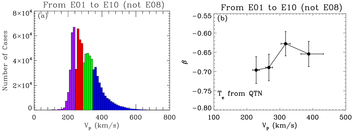
Fig. 5. Power indices as a function of the proton bulk speed. (a) We define the four wind families based on the proton bulk speed histogram. Each colored histogram has the same number of observations. (b) Outcome of the power law modelling in the form T_e = T_0 \times (R/R_\odot)^\beta for total electron temperature: \beta versus V_p . More details are described in the main text.
