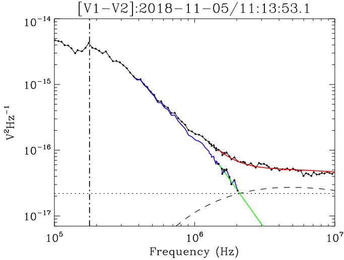
Fig. 1. Example of a voltage power spectrum (between 100 kHz and 10 MHz) recorded by the RFS receiver using the |V1 - V2| dipole electric antennas from FIELDS instrumentation (full black curve connected by crosses). Dot-dashed line gives the position of the local plasma peak (Moncuquet et al. 2020). Dotted horizontal line represents the pre-deployment RFS instrument noise (after launch) of \sim 2.2 \times 10^{-17} \text{ V}^2 \text{ Hz}^{-1} . Black dashed line shows the modelled radio galaxy noise. Blue and green lines represent the effective QTN signal and linear fit ( f^{-3} variation that the QTN spectrum should follow when f \gg f_p L_D / L ), respectively. Black dots on the blue line are used to derive the linear fit. Red line is the sum of the fitted QTN signal, the modelled radio galaxy noise, and the instrument noise. More details are given in the text.
