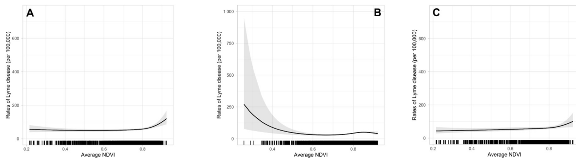
Fig. 3. Subgroup analyses of the associations between rates of Lyme disease and average NDVI and according to calendar year in which rates began to become underestimated (2013) as well as in different states. A Lyme disease rates and average NDVI for the years 2000–2012. B Lyme disease rates and average NDVI for the years 2013–2018. C Lyme disease rates and average NDVI for the years 2013–2018 but excluding New York State, Maryland, Minnesota, and Connecticut.
