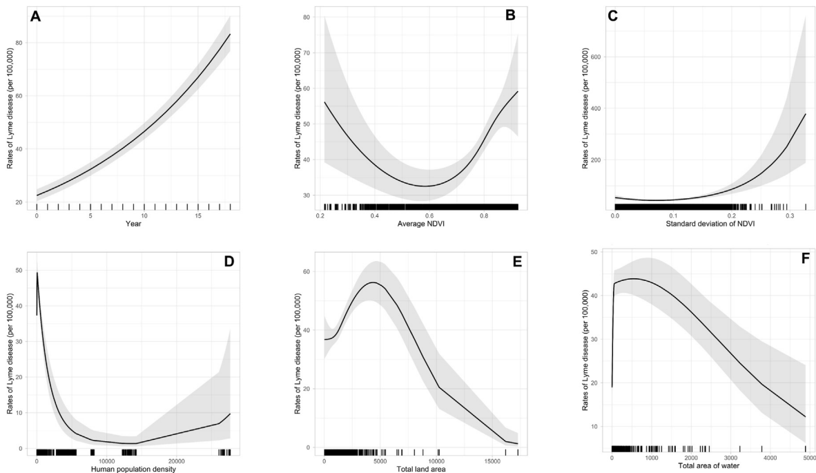
Fig. 1. Predicted rates of Lyme disease from a quasi-Poisson regression model that included year as a linear term, and natural cubic splines for average NDVI, the standard deviation of NDVI, population density, area of water, and total area of the county for the years 2000–2018, including 580 counties in 15 states (11,020 observations). Three degrees of freedom were used for all variables except for standard deviation of NDVI ( df = 2 ). The solid line represents the predicted value and the grey area surrounding the line represents the pointwise 95% confidence interval. The rug plot (tick marks) on the x-axis represents the location of the data points. A Response function for year. B Response function for average NDVI. C Response function for standard deviation of NDVI. D Human population density. E Total land area of the county. F Total area of water.
