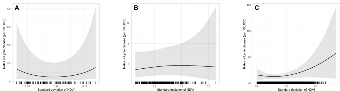
Fig. 2. Interaction analysis of standard deviation of NDVI and rates of Lyme disease. Interaction between average NDVI and standard deviation of NDVI adjusted for other covariables. Average NDVI was split into 3 categories. Category 1 includes average NDVI from 0 to 0.4. Category 2 includes average NDVI from 0.4 to 0.6. Category 3 includes average NDVI from 0.6 to 1.0. For each category of average NDVI, the fitted response curves of the interaction analysis are shown. A Lyme disease rates and standard deviation of NDVI. Category 1 (0–0.4). B Lyme disease rates and standard deviation of NDVI. Category 2 (0.4–0.6). C Lyme disease rates and standard deviation of NDVI. Category 3 (0.6–1.0).
