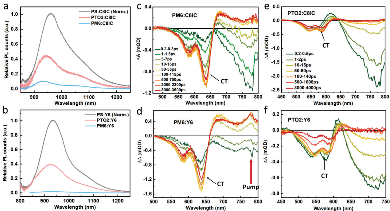
Figure 3. a,b) Steady-state PL quenching of the blends with respect to the neat films. The excitation is a continuous light \lambda_{exc} = 780 nm with intensity \leq 100 mW cm ^{-2} . The PL intensities of the films are calibrated by their absorptions at 780 nm. Transient absorption (TA) spectra in the visible region conducted on c) PM6:C8IC, d) PM6:Y6, e) PTO2:C8IC, and f) PTO2:Y6 with a pump at 760 nm ( \leq 4 \mu J cm ^{-2} ). The 2D TA spectra are shown in Figure S7, Supporting Information.
