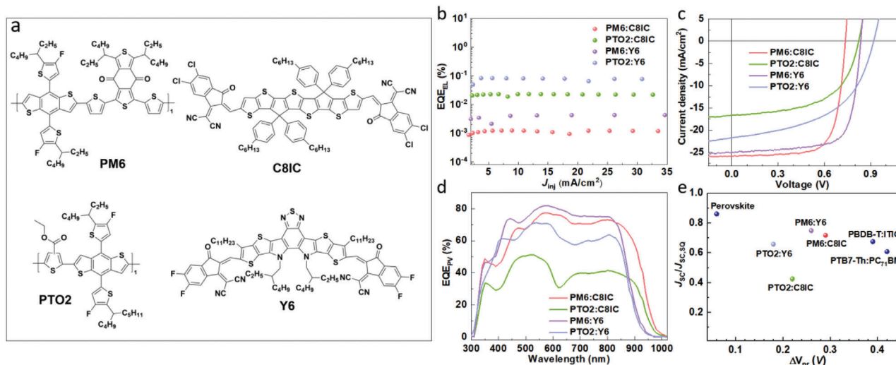
Figure 1. a) Chemical structures of the electron donors (PM6 and PTO2) and electron acceptors (C8IC and Y6) studied in this work. b) \text{EQE}_{\text{EL}} as a function of injected current density, c) current-voltage ( J - V ) characteristics, and d) \text{EQE}_{\text{PV}} spectra of the devices based on PM6:C8IC, PTO2:C8IC, PM6:Y6, and PTO2:Y6. The \text{EQE}_{\text{EL}} values of the devices are extracted from (b), where the injected current densities ( J_{\text{inj}} ) are comparable to the short-circuit current densities of the devices. e) Charge generation efficiency ( J_{\text{sc}}/J_{\text{sc,SQ}} ) versus \Delta V_{\text{nr}} .
