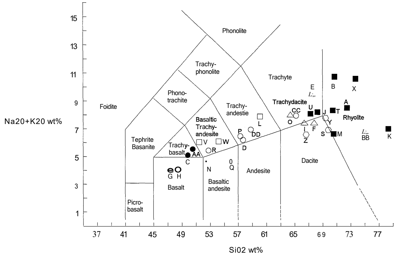
Figure 6. Total alkalis vs. SiO 2 for rocks from western and central Gila Bend and southern Eagletail Mountains, Maricopa and Yuma Counties, Arizona. • - unit Tb; ○ - unit Tm; L v - felsic volcanic rocks (Tf, Tfv, Tt); ■ - unit Tg; □ - unit Tmd; ○ - unit YXgn. Classification scheme for volcanic rocks from Le Bas and others (1986). Map symbols A-S reported in Gilbert and Spencer (1992) and Gilbert and others (1992), symbols T-DD in this report.
